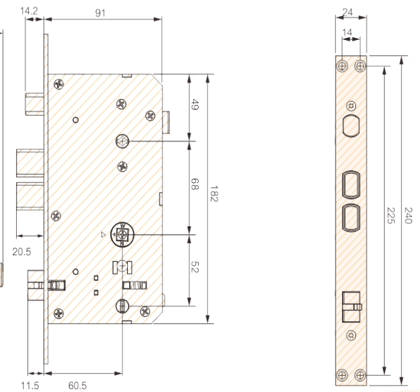
Lock Body (Unit: mm)
