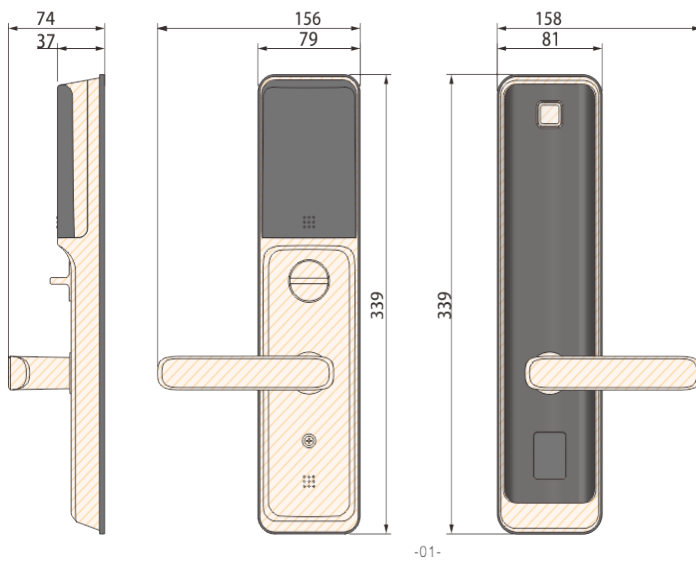
Panel (Unit: mm)
